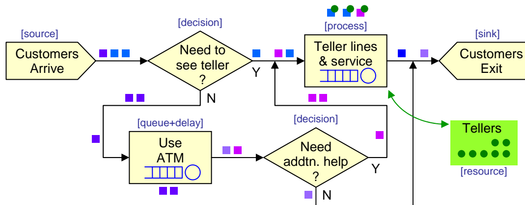
Figure 6: Discrete Event Model: Bank Kiosk in Arena™
