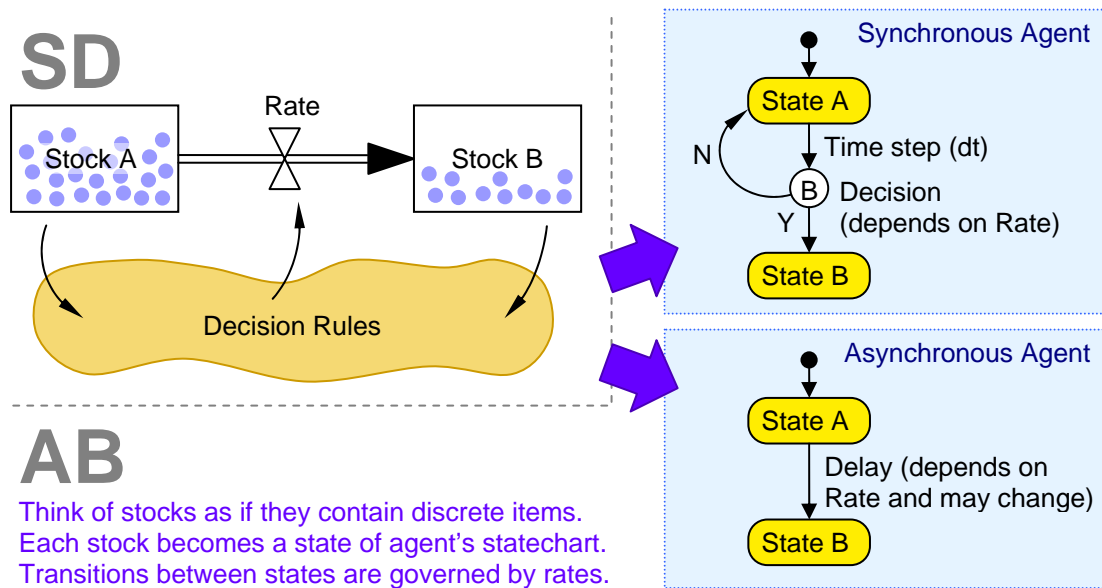
Figure 9: Re-Conceptualizing a System Dynamics Model into Agent Based Model. General Scheme
