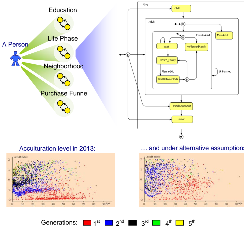
Figure 18: Agent Based Model of Dynamics of Hispanic Population Acculturation and Behavior
