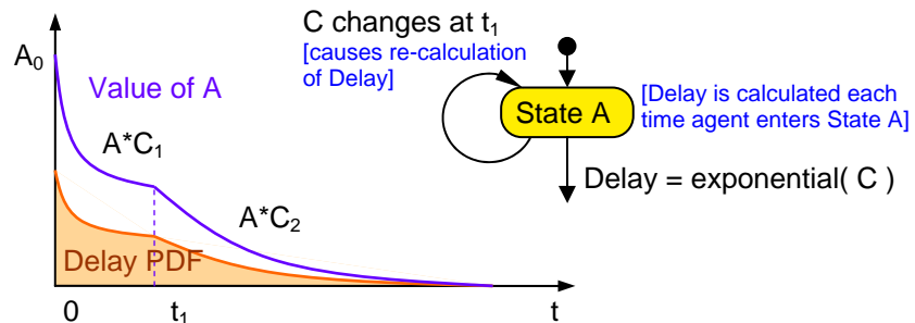
Figure 20: Correspondence of SD and AB Models. Constant and Proportional Rates
