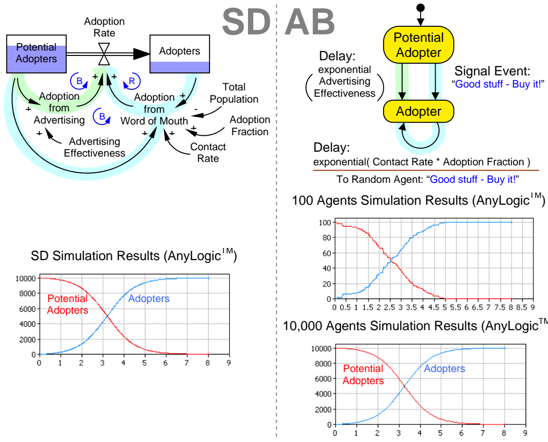
Figure 10: Bass Diffusion Model Converted From System Dynamics to Agent Based
